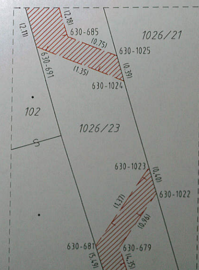
detail "H"
