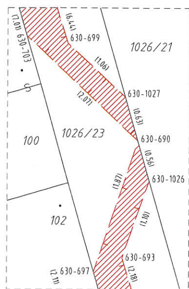
detail "K"
