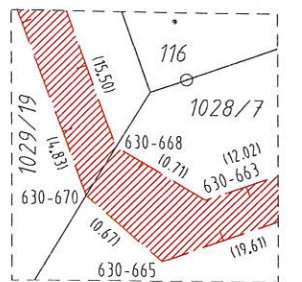
detail "E"
