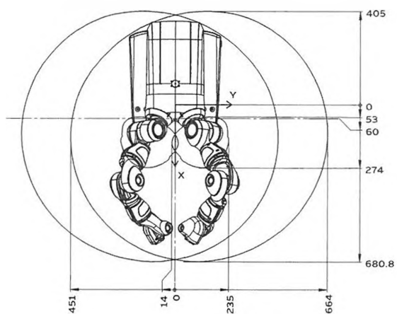
IRB 14000-0.5/0.5 Pohled shora
