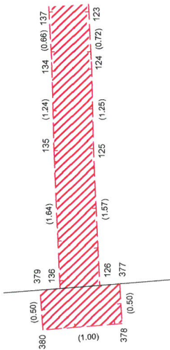
DETAIL E:
