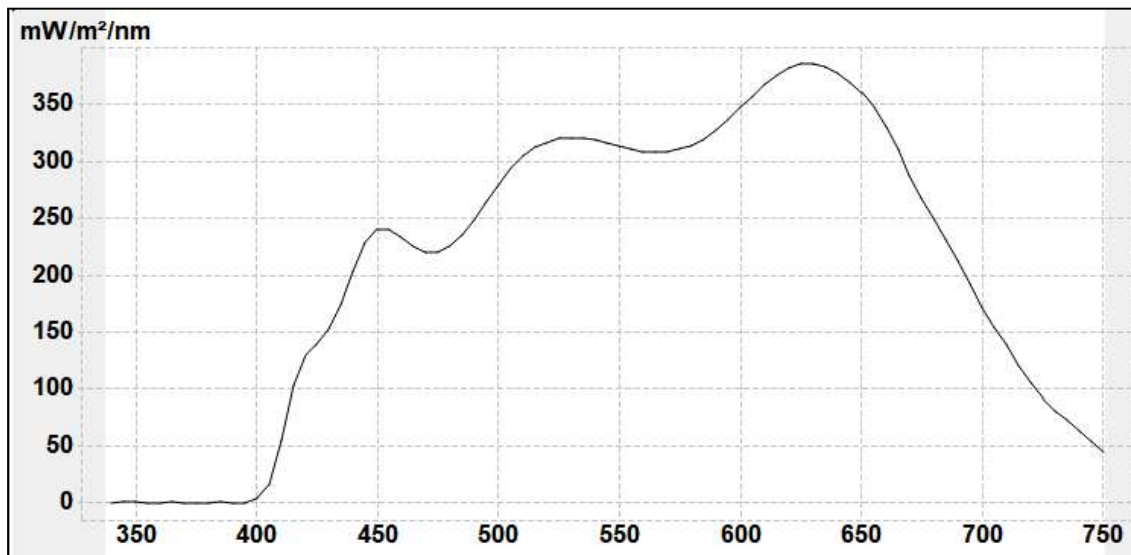
Spectral response True Daylight PLUS
