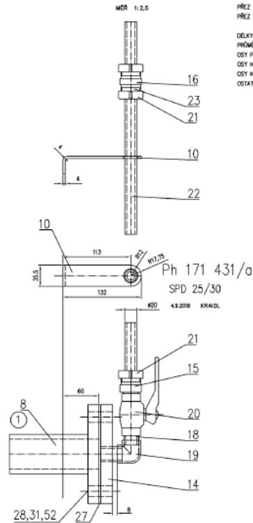
DETAIL A
