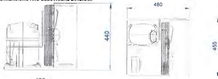
DIMENSIONS AND ELECTRICAL DIAGRAM
