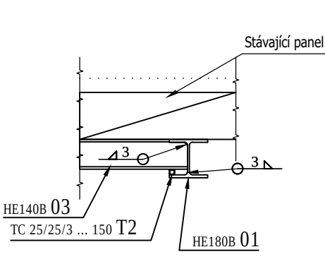
DETAIL "D" 1:25 celk. 6x
