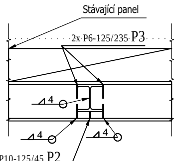
DETAIL "B" 1:25 celk. 21x
