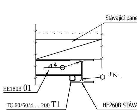
DETAIL "C" 1:25 celk. 8x
