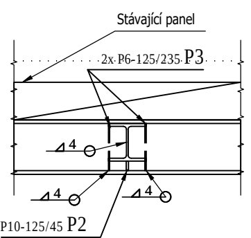
DETAIL "B" 1:25 celk. 8x
