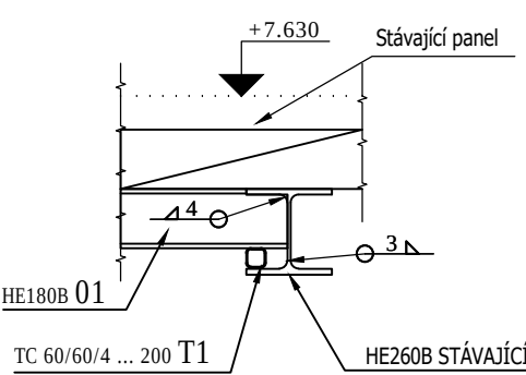
DETAIL "C" 1:25 celk. 8x
