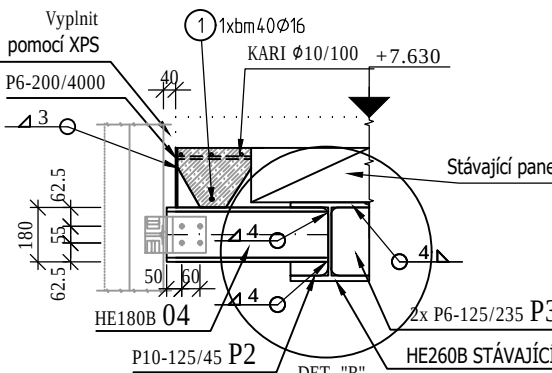
DETAIL "A" 1:25
