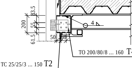
DETAIL "G" 1:25 18x
