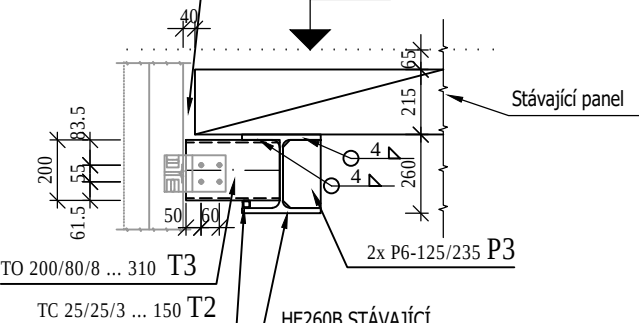
DETAIL "F" 1:25 24x
