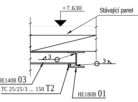
DETAIL "D" 1:25 celk. 6x
