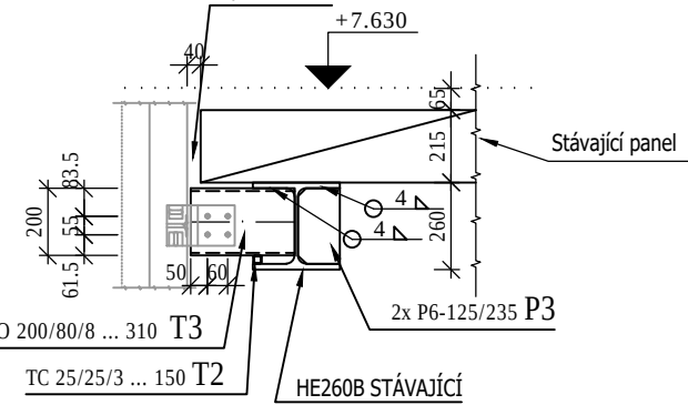
DETAIL "F" 1:25 17x
