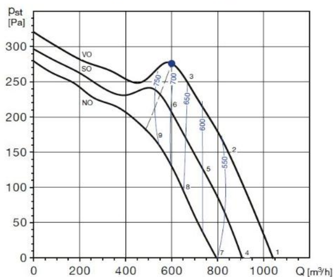
TD-1000/200 SILENT 3V
