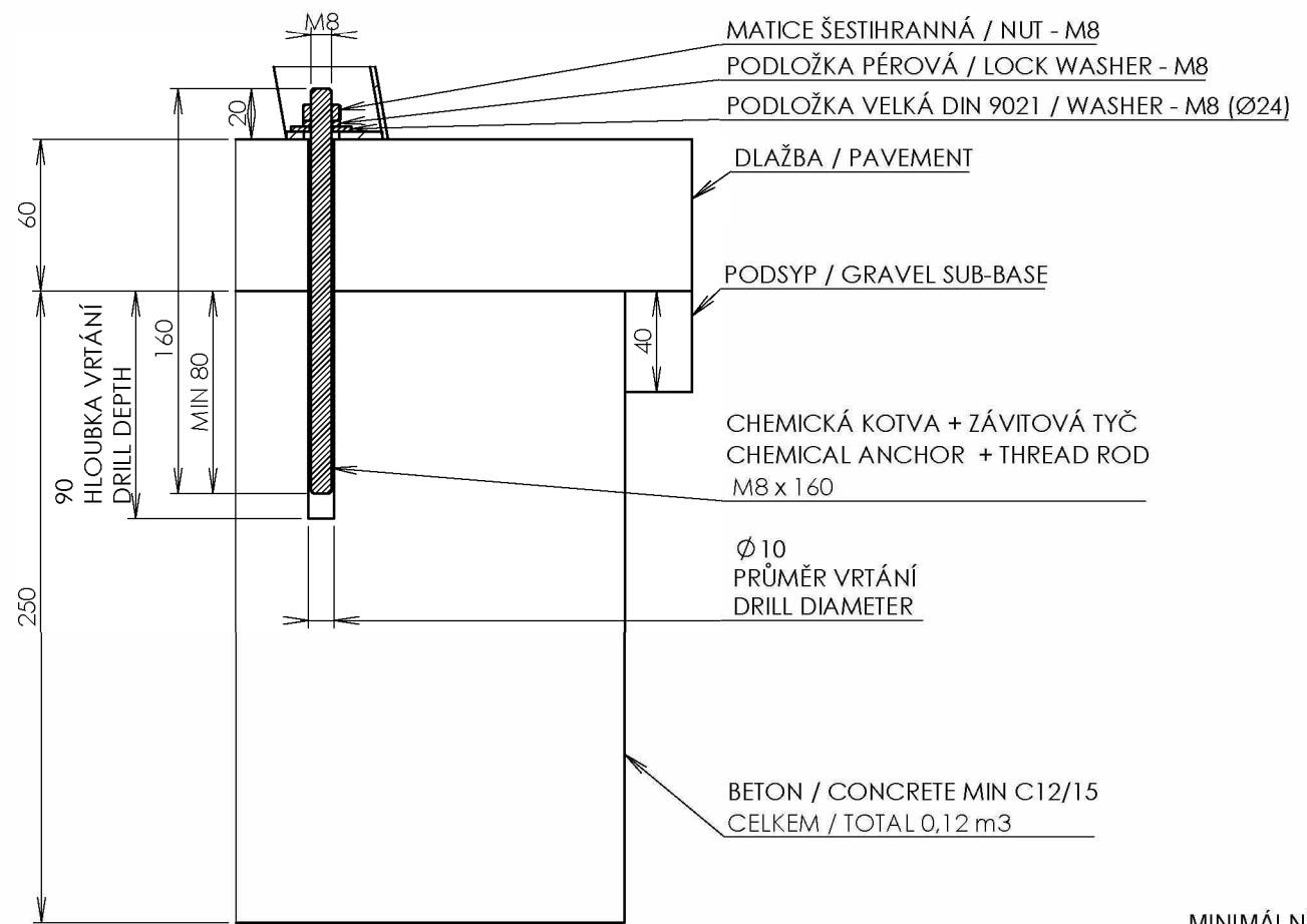
DETAIL Z
