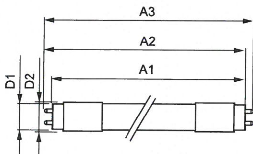
MASTER LEDtube 1500mm UO 21.7W 840 T8
