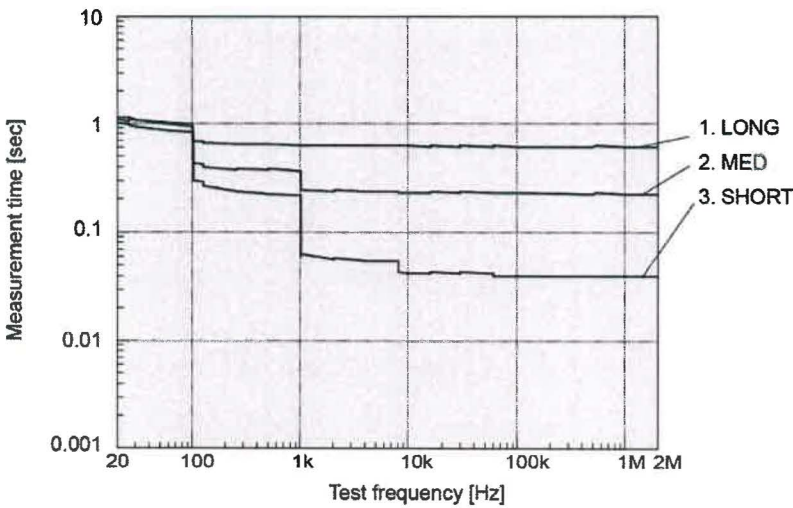
Figure 10. Measurement time (E4980BL)
