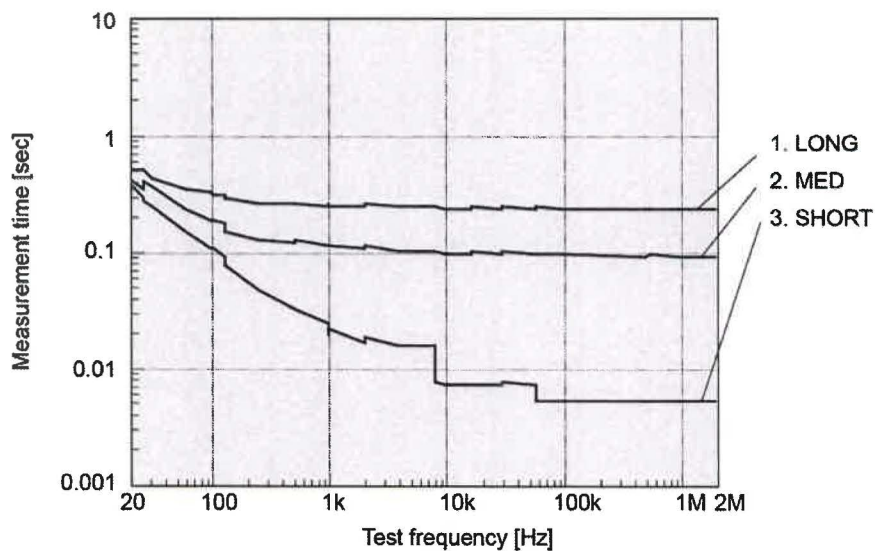
Figure 9. Measurement time (E4980B, DC bias: OFF)
