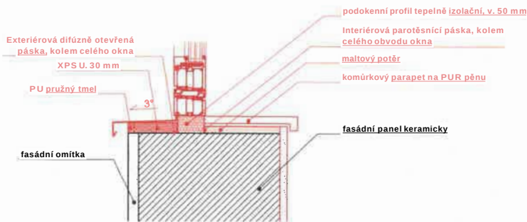
AD Detail parapetu 1:10
