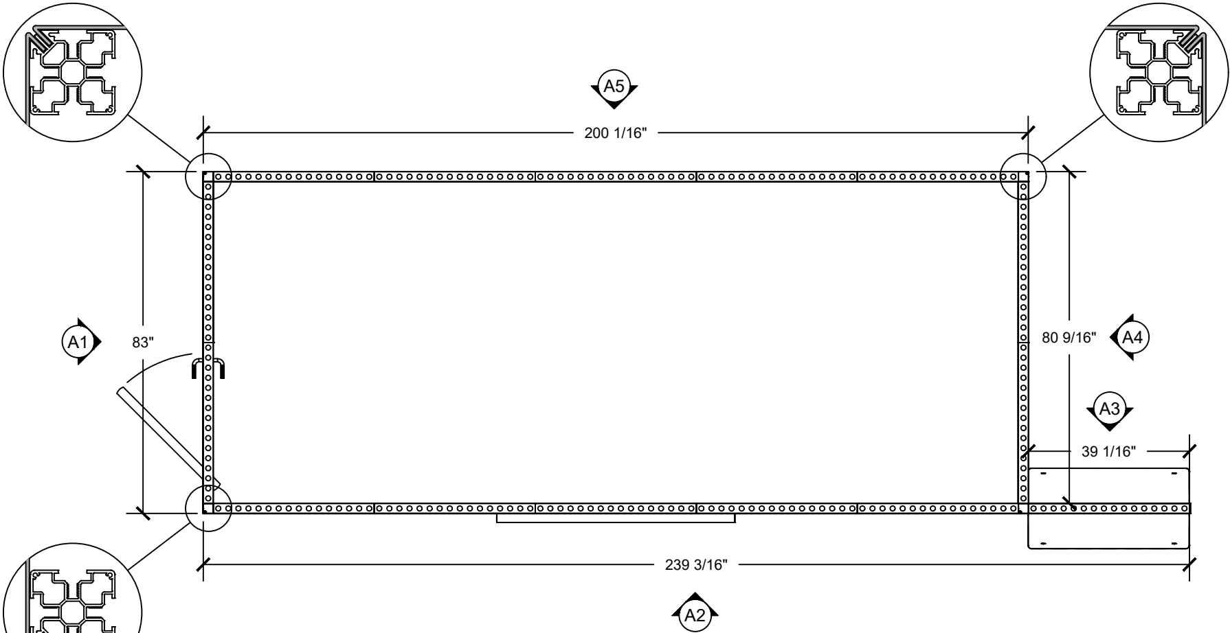
PLAN VIEW - FABRIC
