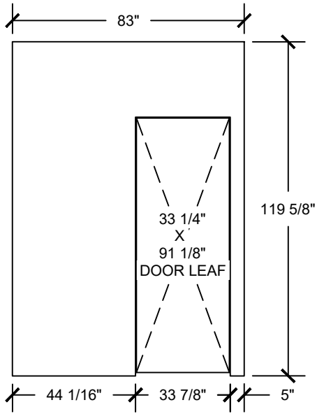
FLAT VIEW - FABRIC "A1"
