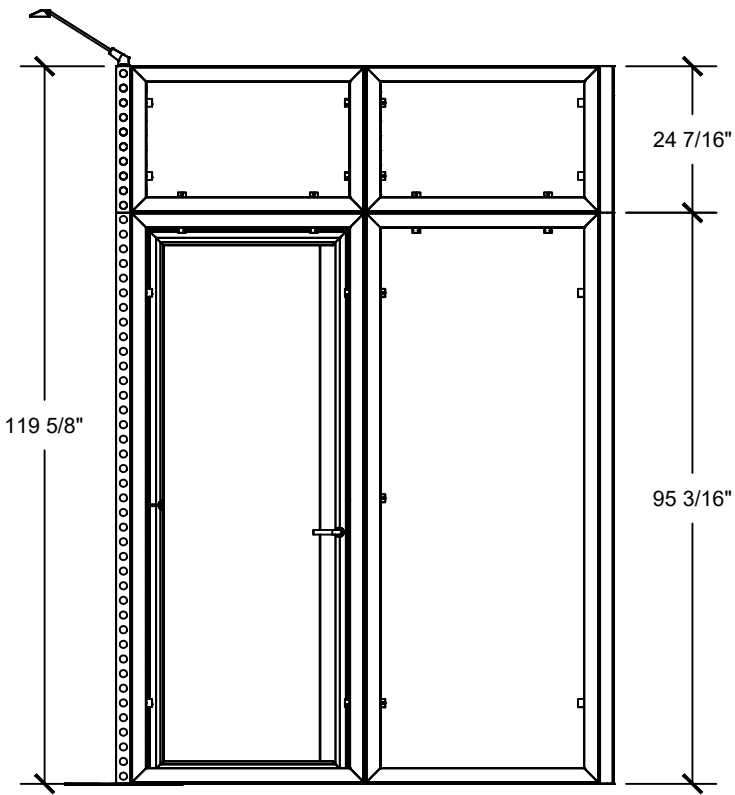
ELEVATION VIEW "B"
