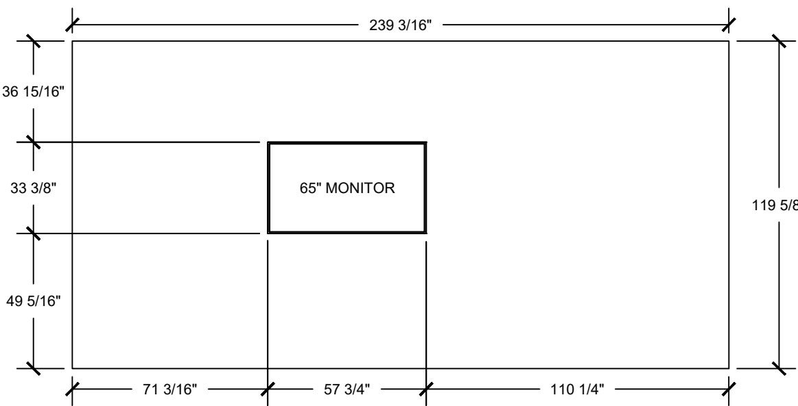
FLAT VIEW - FABRIC "A2"
