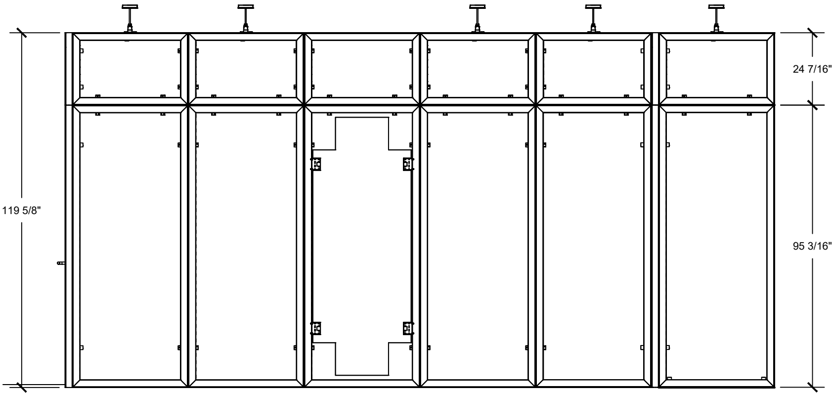
ELEVATION VIEW "A"
