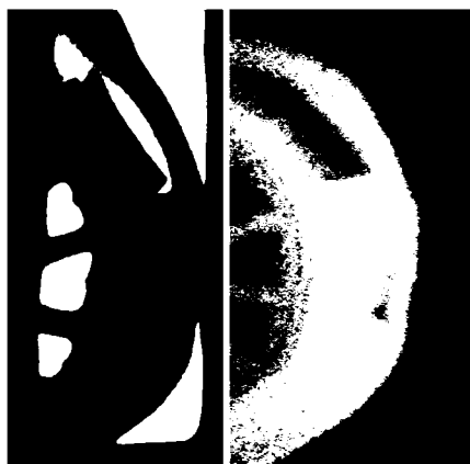
The transmission image (left) reveals a lead box (used to conceal narcotics) welded to a tire rim. The Z Backscatter image (right) highlights drugs placed in the tire itself.
