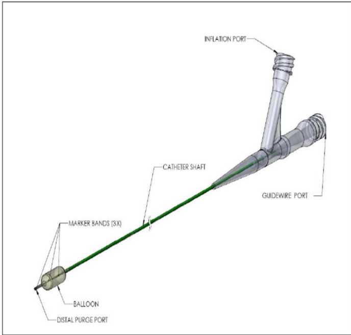
Scepter C and XC Balloon Catheter Diagram
