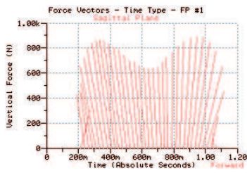
Fig. 6: Force vector
