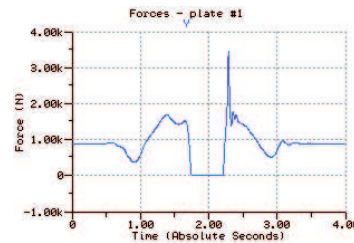
Fig. 7: Jump force
