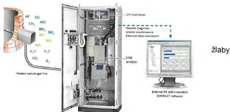
Obr. 1 Systém MCS200HW
