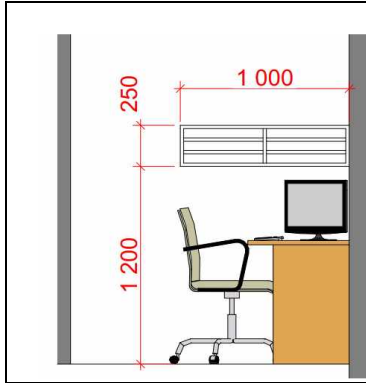
Pohled P05
