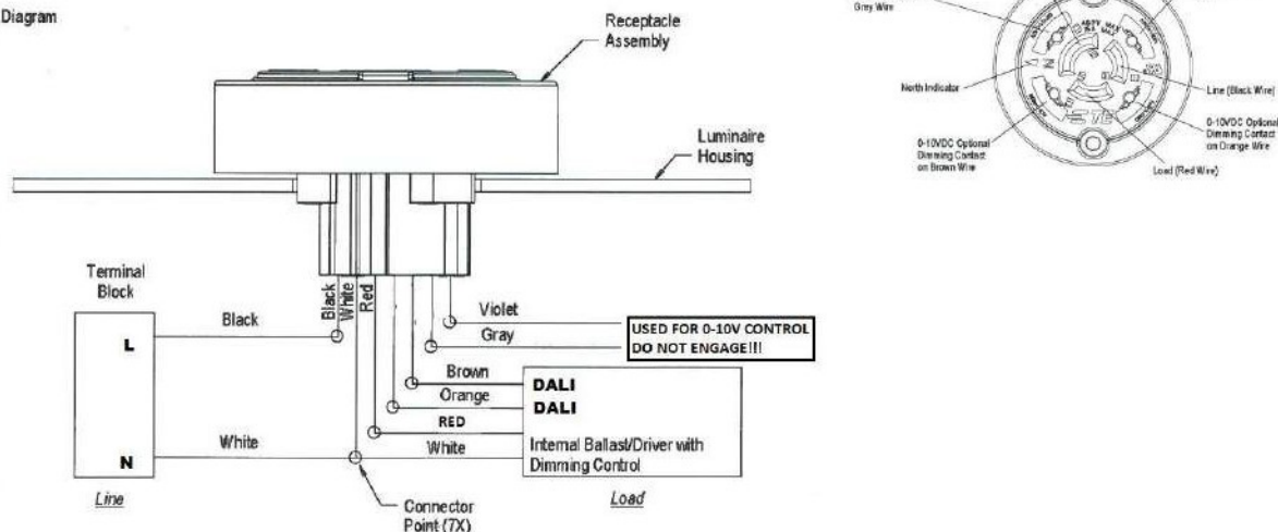
Wiring Diagram
