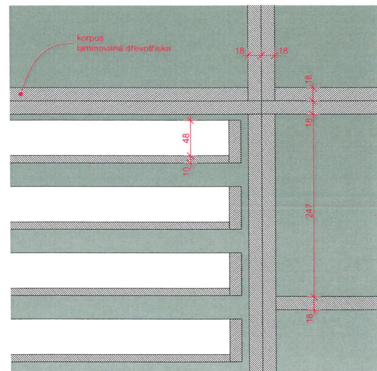
detail D4
