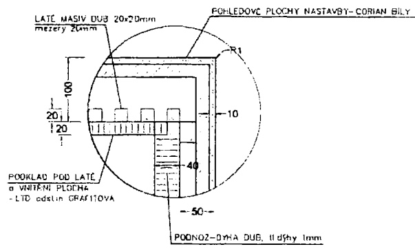
detail X
