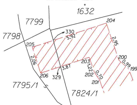
Detail E:
