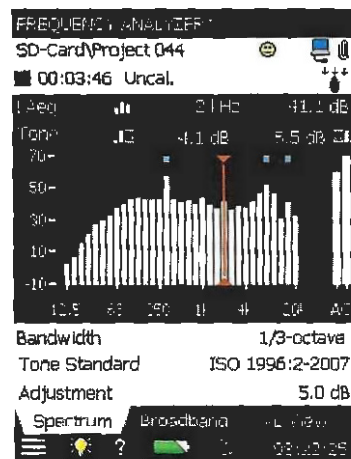
Fig. 11 Tone Assessment Option BZ-7231 showing 1/3-octave bands with audible tones higher than a set limit (tones are identified by the blue dots)
