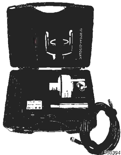
Fig. 9 Two-parameter Weather Station Kit MM-0316-A
