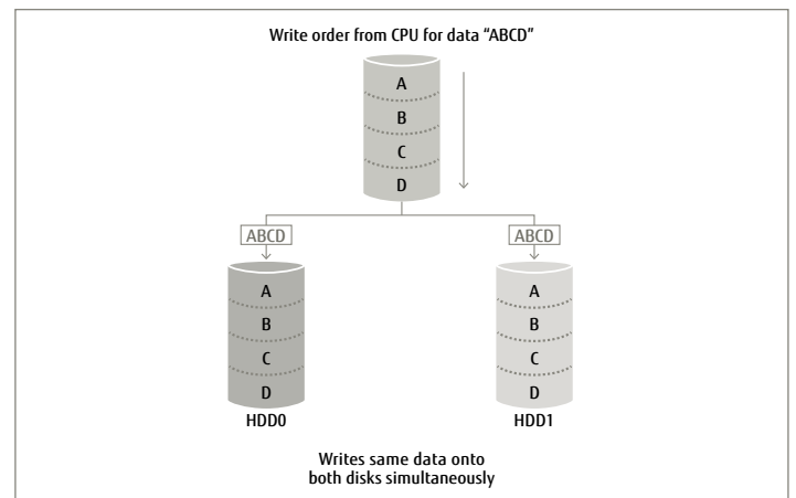
RAID 1
