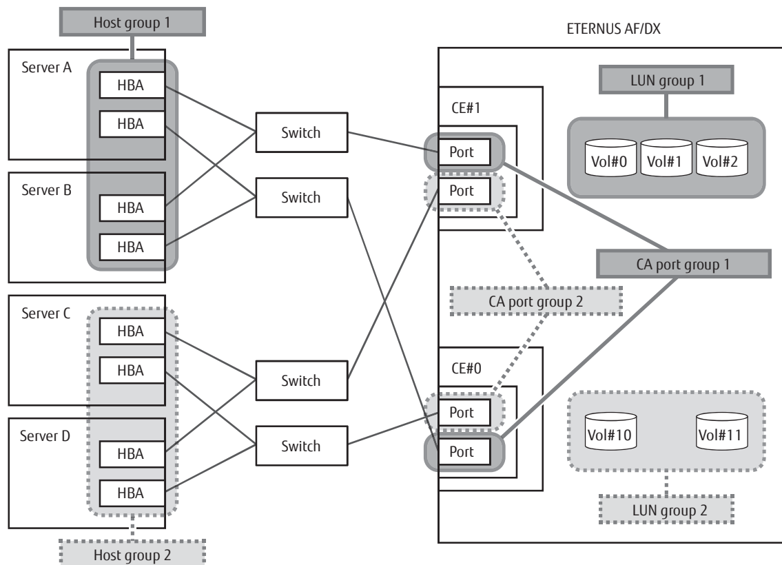
Figure 3 Host affinity settings (association of host groups, port groups, and LUN groups)
