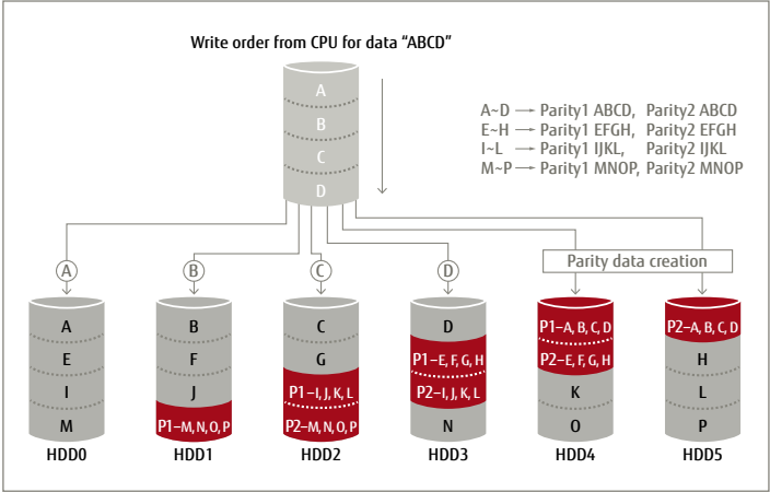
RAID 6
