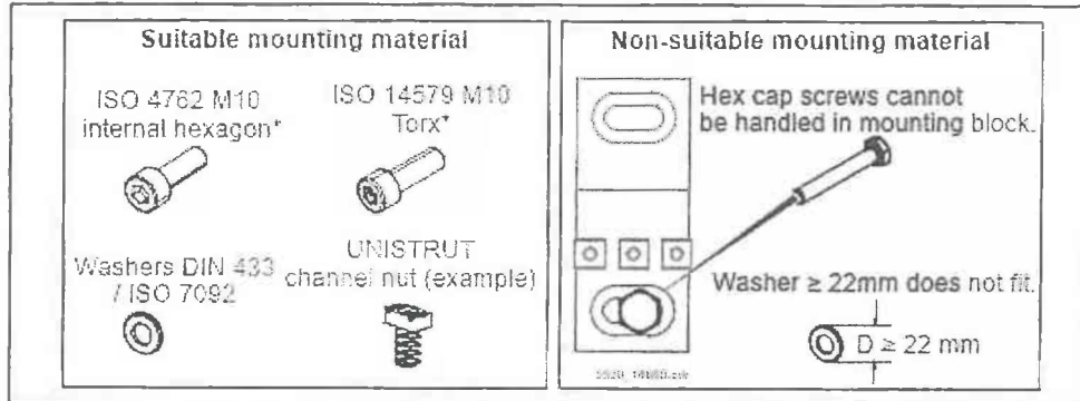
Figure 19: Mounting material
