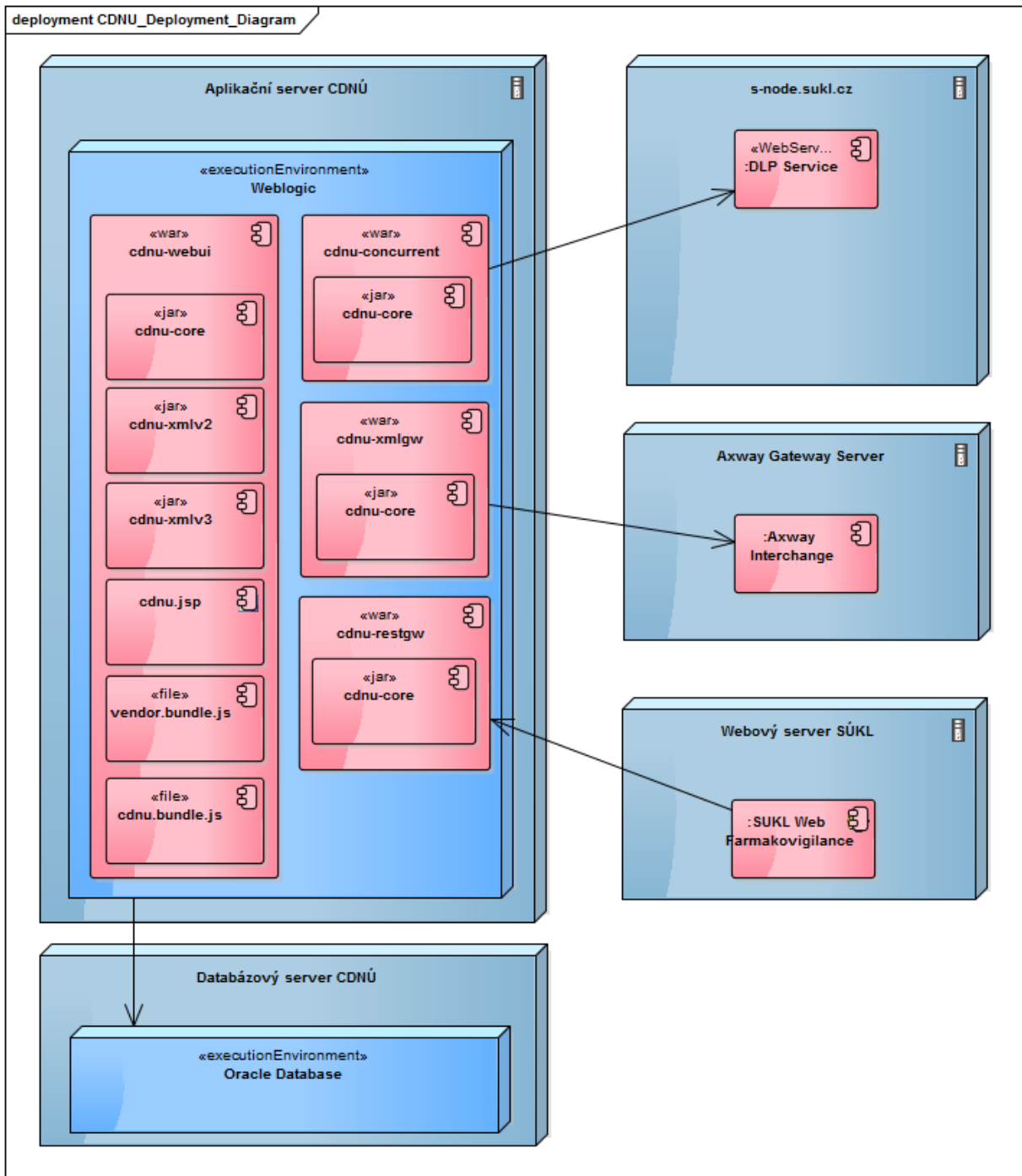
CDNU_Deployment_Diagram
