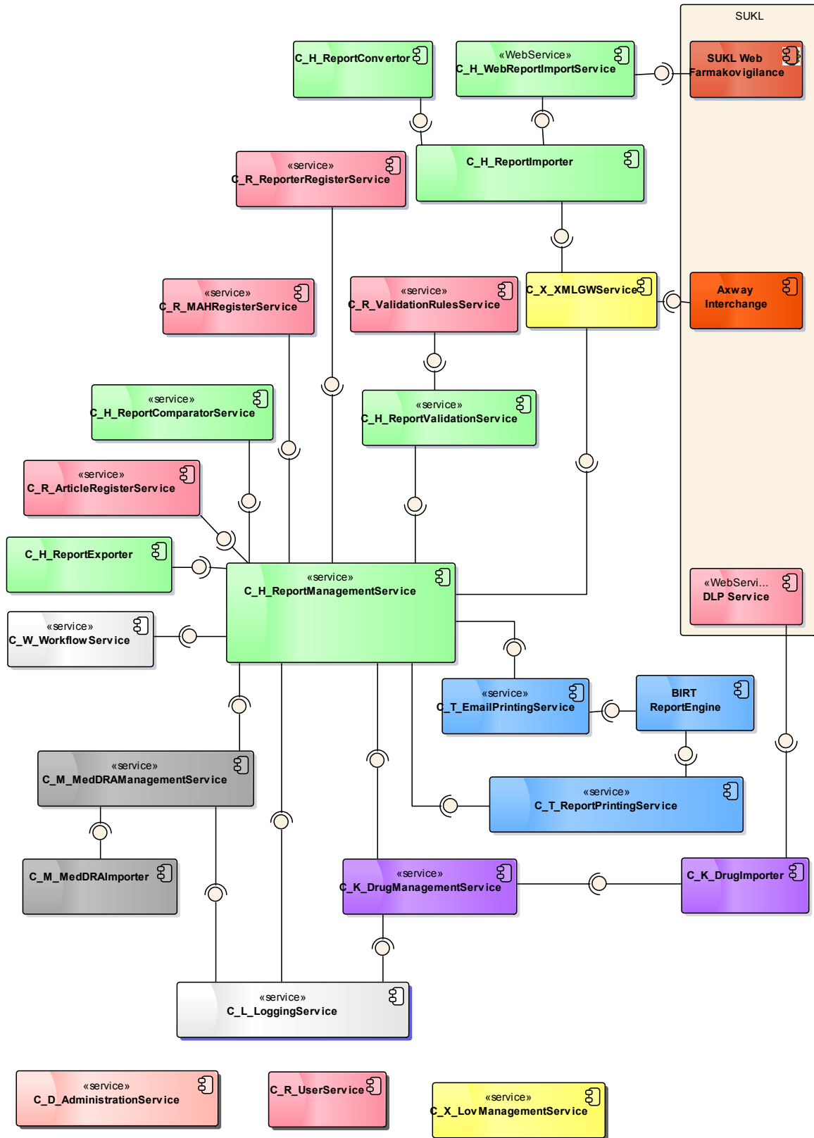
CDNU_Detail_Component_Diagram
