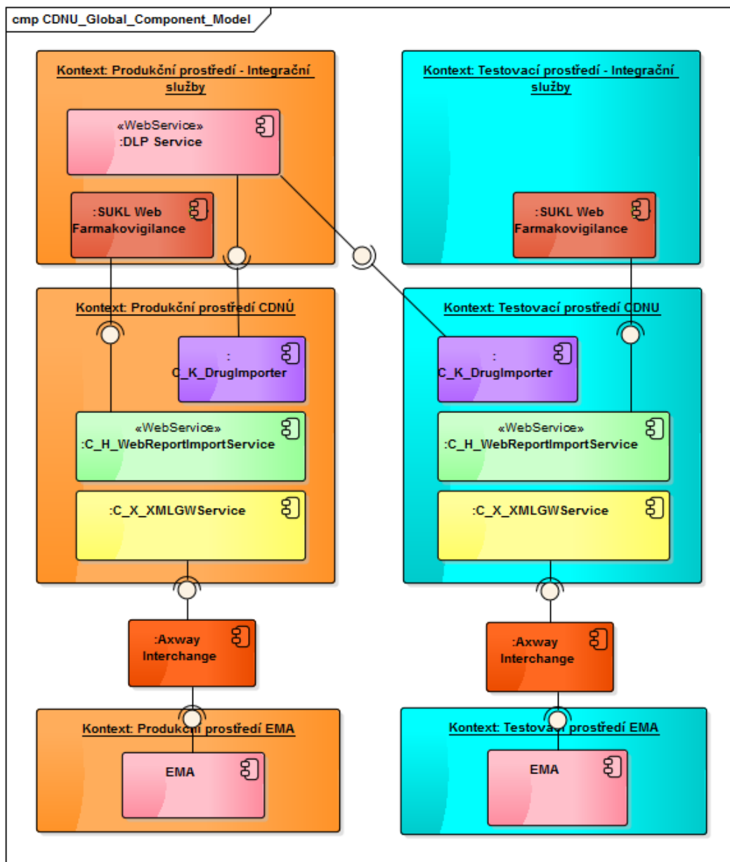
CDNU_Global_Component_Model
