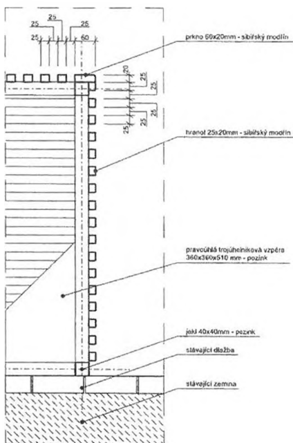
detail lavice 1:10
