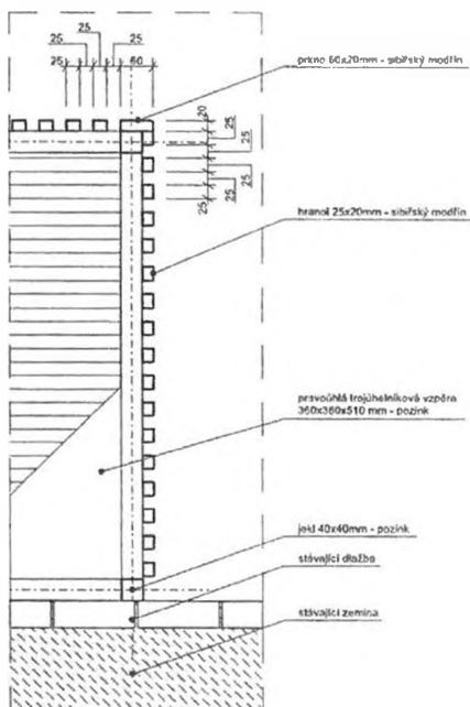
detail lavice 1:10
