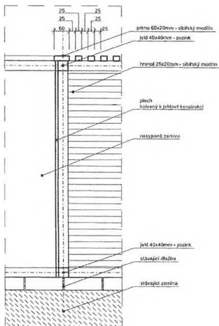
detail lavice 1:10
