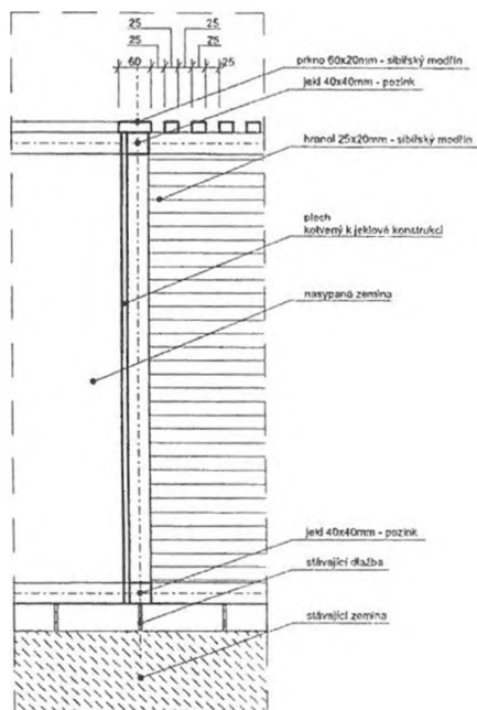
detail lavice 1:10
