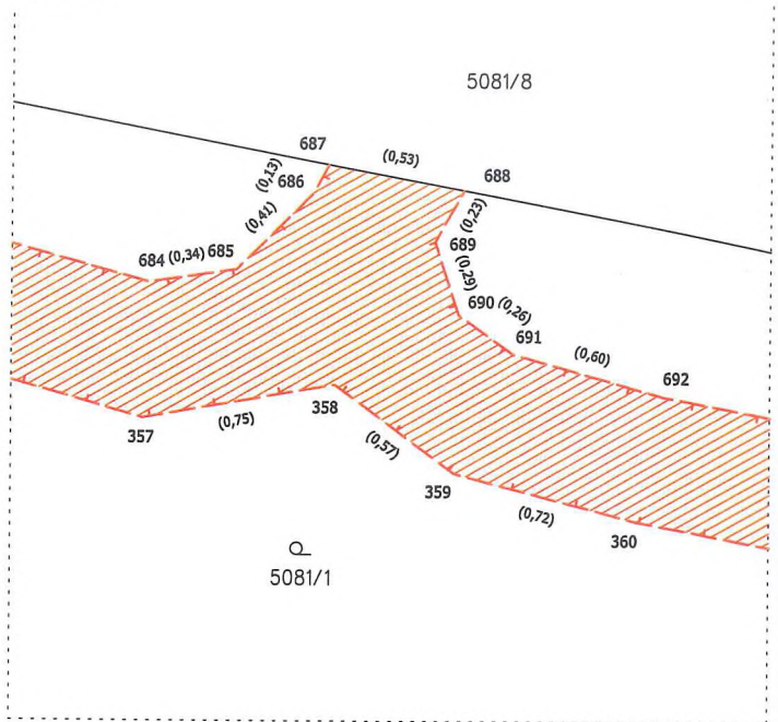
Detail H
