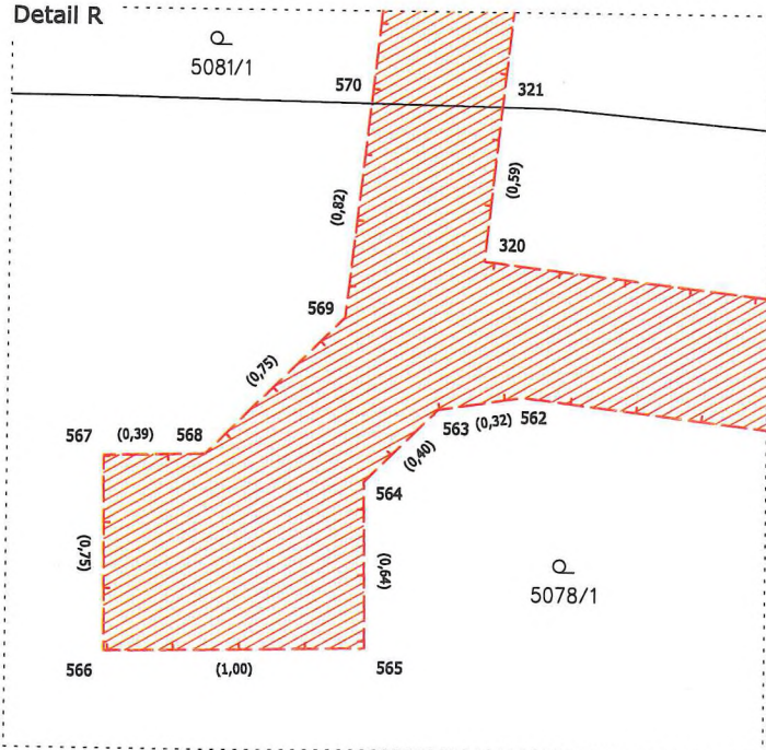
Detail R
