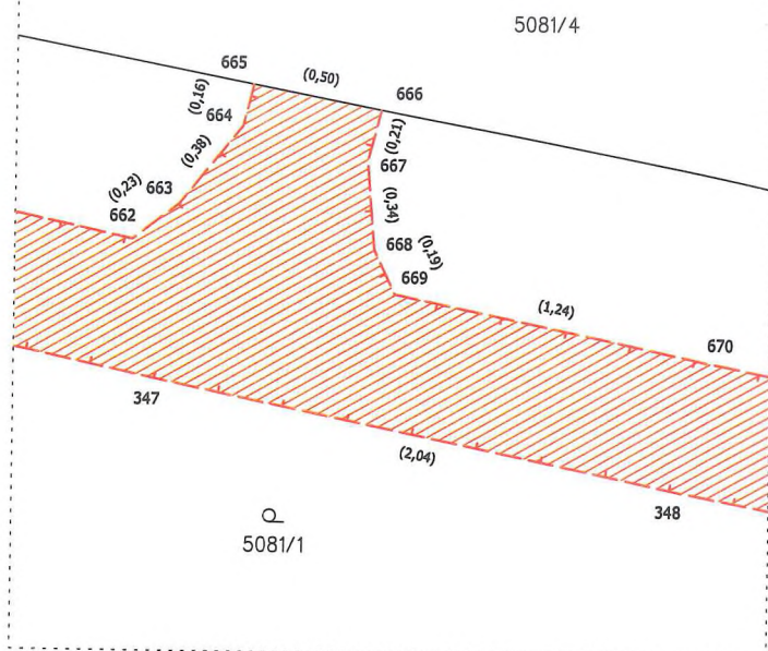
Detail P
