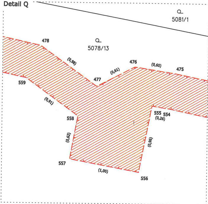
Detail Q
