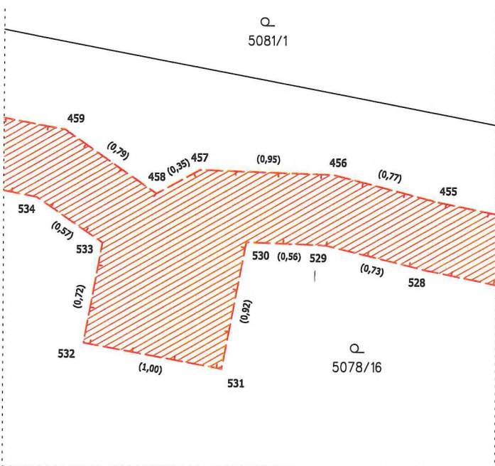
Detail K
