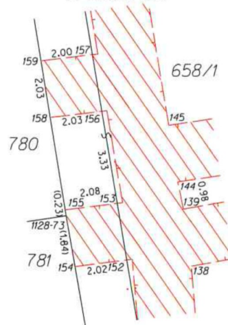
Detail D:
