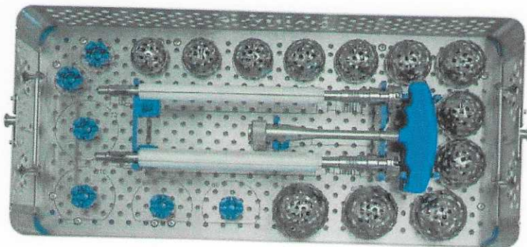
Acetabular Reamer Instrumentation, 51.34.1081A
