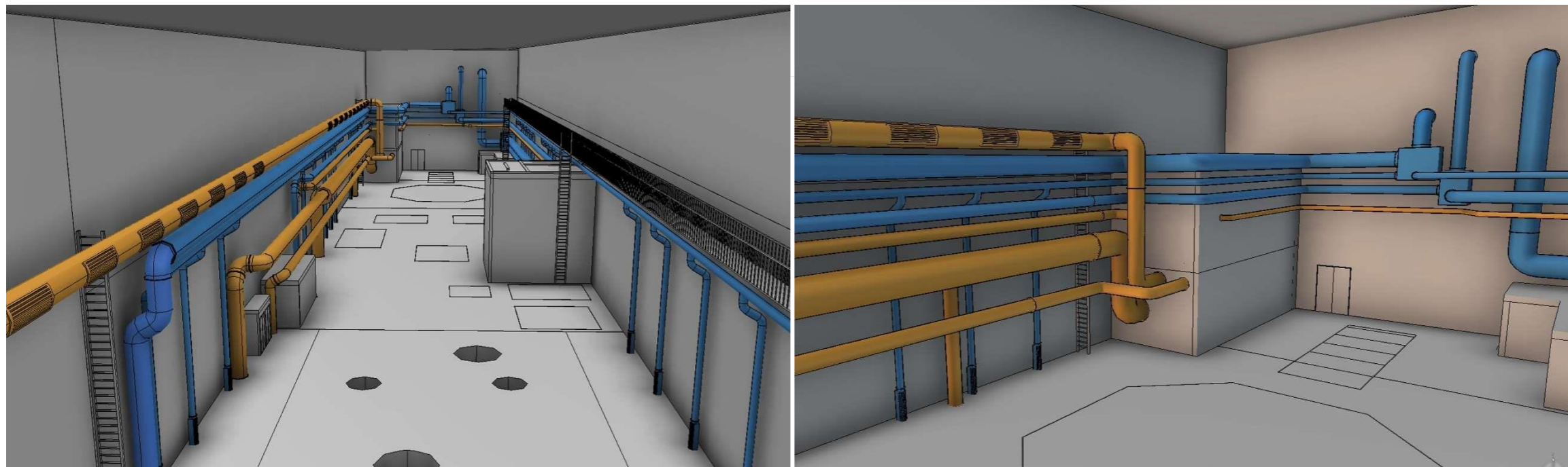
Figure 5: detail of the ducts routing inside the High Bay
