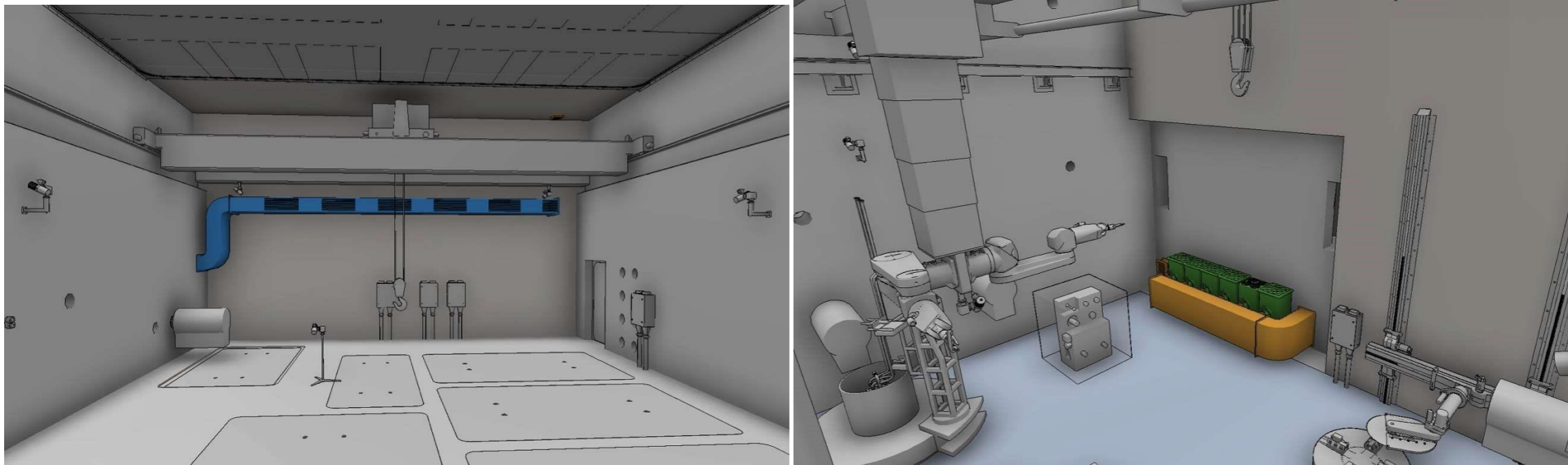
Figure 4: Detail of the duct layout inside the Process Cell
