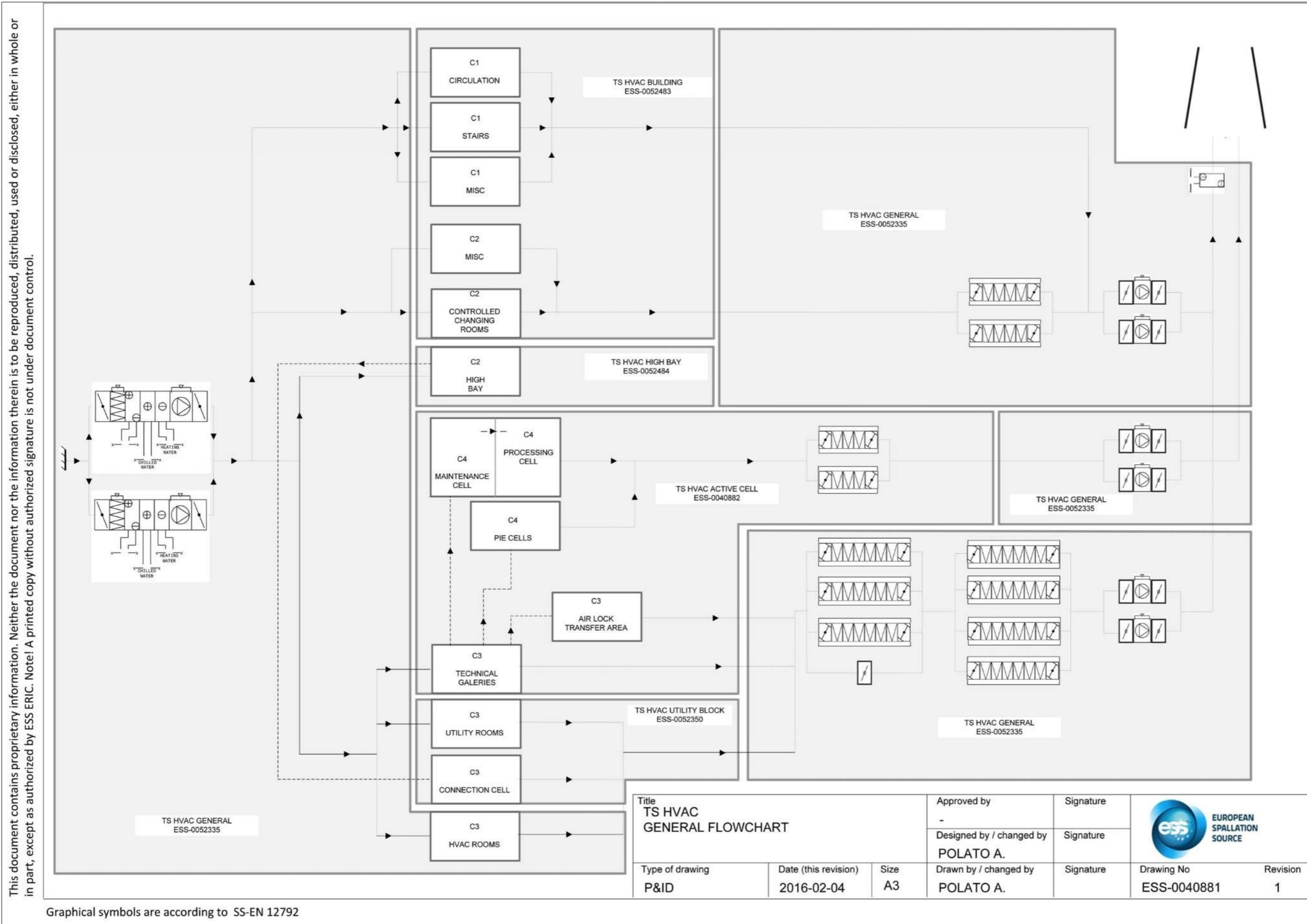
Figure 1: TS HVAC flowchart
