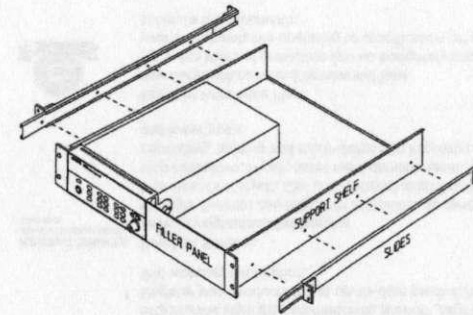
To install one or two instruments in a sliding support shelf, order shelf 5063-9255, and slide kit 1494-0015 (for single instrument, also order filler panel 5002-3999).
