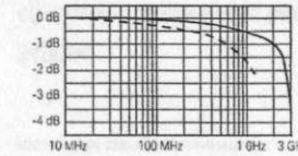
Insertion loss
