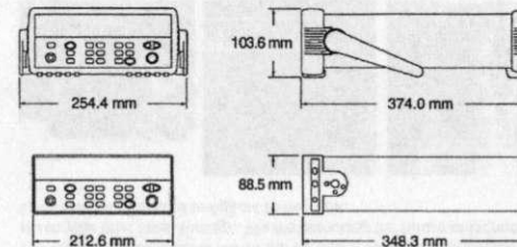
To install one or two instruments in a sliding support shelf, order shelf 5063-9255, and slide kit 1494-0015 (for single instrument, also order filler panel 5002-3999).
