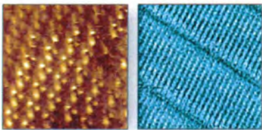
Self-assembled monolayers. Left: Octadecan-1-thiol, scan size: 6 nm. Right: Dotriacontane, scan size 13 nm.
