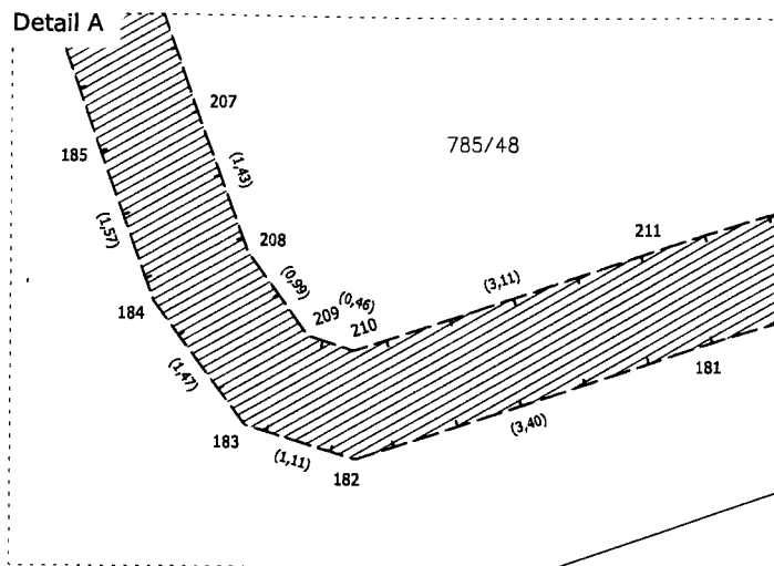
Detail C
