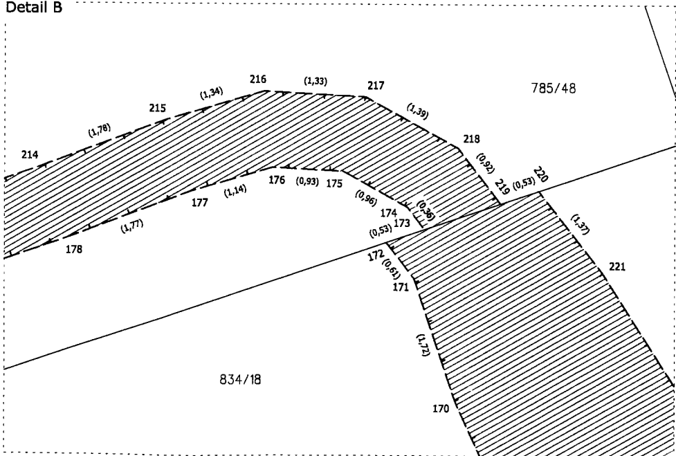
Detail B
