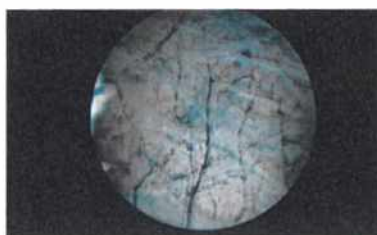
Spectra A
