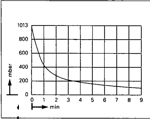
Pump down time for 5 l receiver
